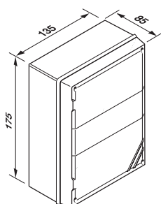
T21X - T21B
