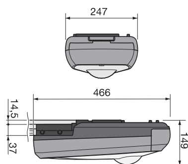
GL124EBSS
